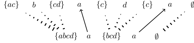
Figure 2: Two sub-observations with a map m satisfying \preceq
