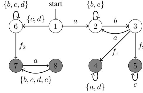
Figure 4: Underlying system of the illustrative example.
