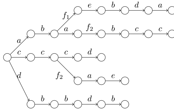
Figure 1: Log tree of L
